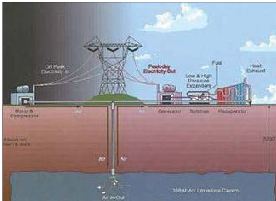
Gas-fired Compressed Air Energy Storage (CAES) System
